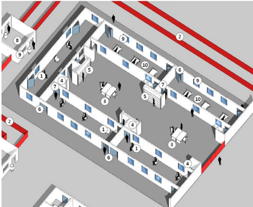
Figure 36. Short-stay and moderate wards in a severe acute respiratory infection treatment centre
